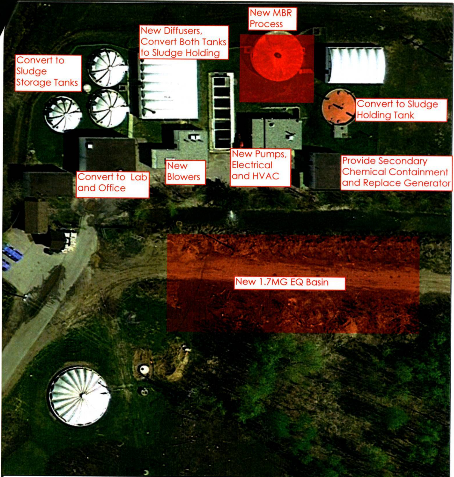
Figure 4: Option 3 (MBR) - WWTF Improvements
