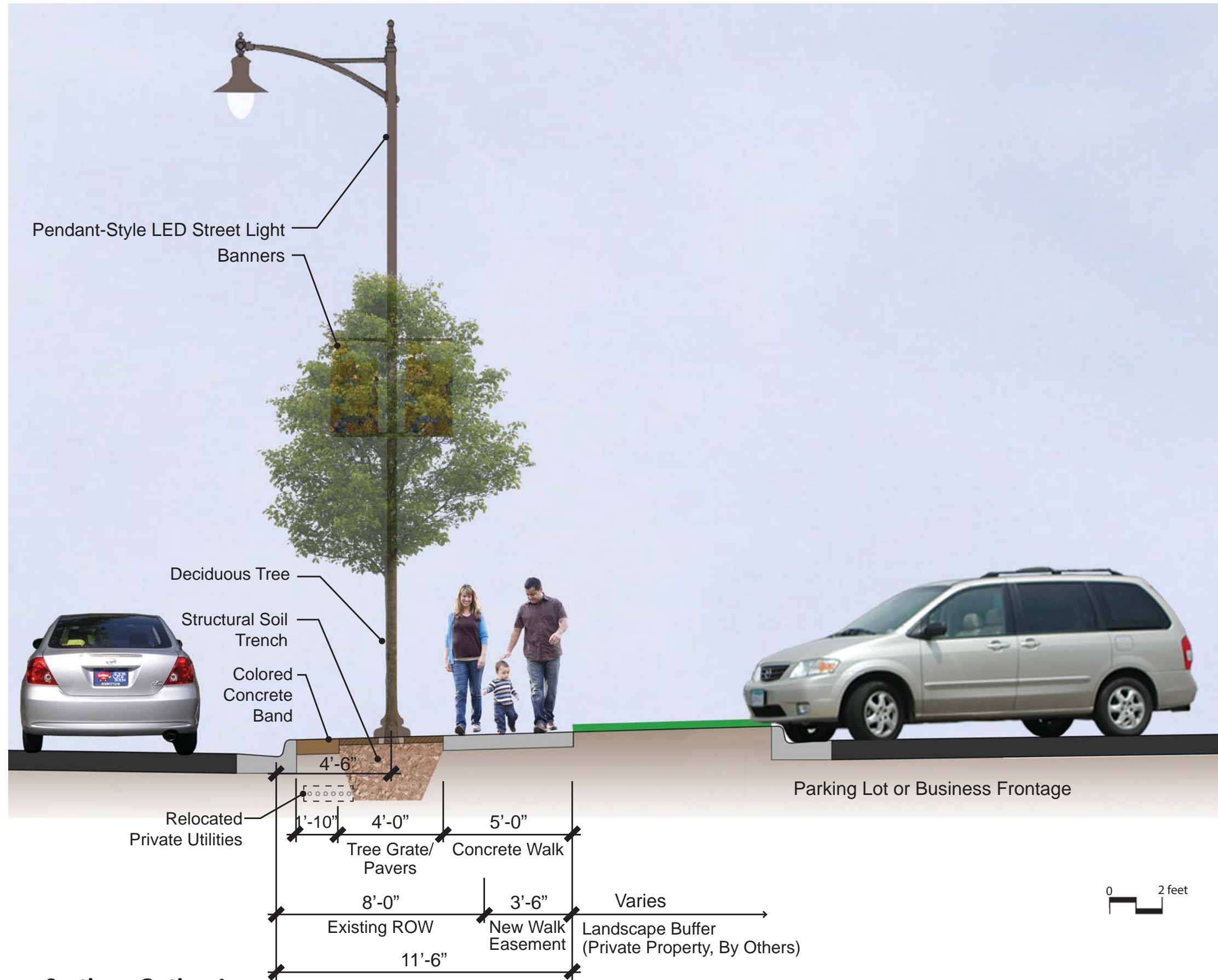
Sidewalk Detailed Cross Section - Option 1
