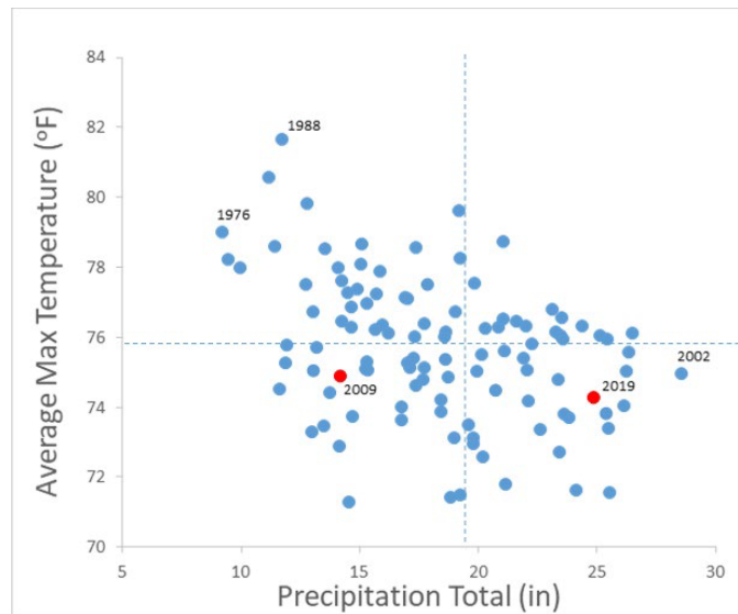
Figure 6. Characterization of air temperature and rainfall conditions for May-September period across the historical record of climate data for the Mississippi River-St Cloud Watershed. Dashed lines represent normal (1991-2020) maximum temperature and total precipitation values for the watershed. IWM years highlighted in red.
